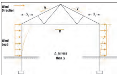
(b) With diaphragm action.
