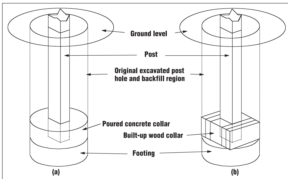
Figure 13. Embedded pressure preservative-treated wood post foundation with concrete footers and: (a) attached concrete collar and (b) attached pressure preservative-treated wood cleats.
