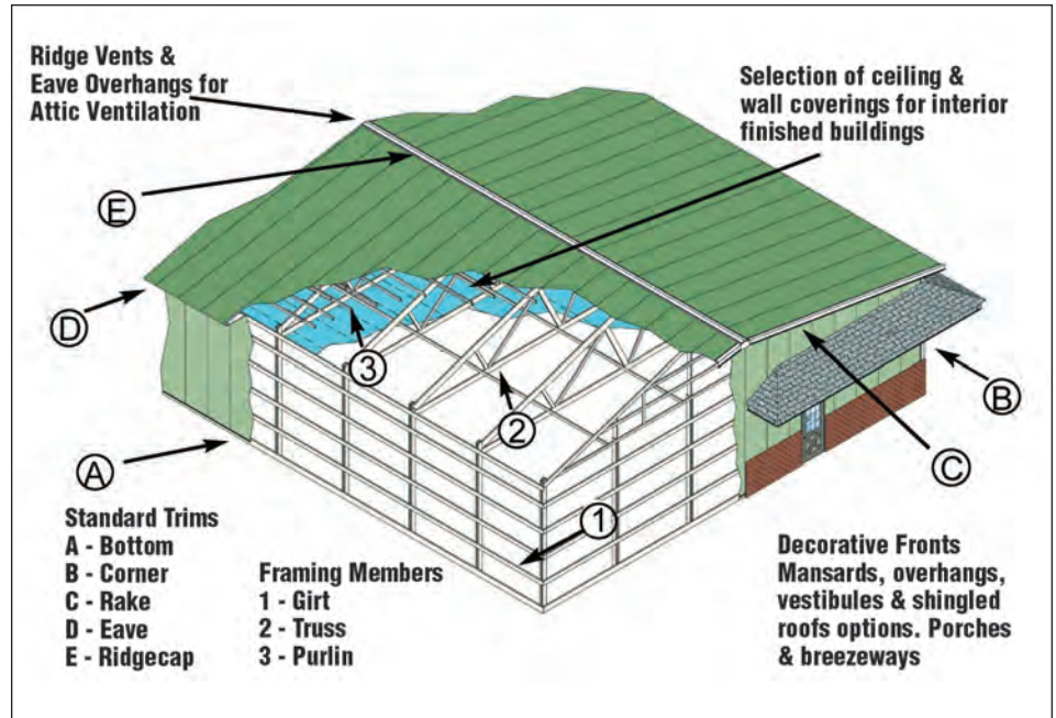
Figure 9. Illustration of typical post-frame building features.
