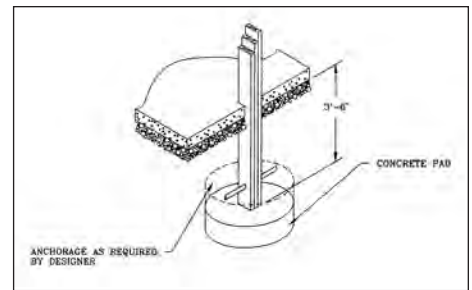
Figure 14. Treated posts may be embedded in the ground.
