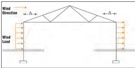
(a) Without diaphragm action.
