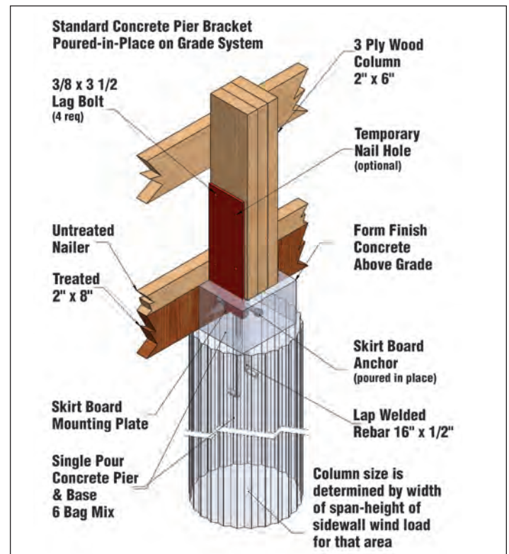
Figure 28. Cast-in-place concrete pier system
