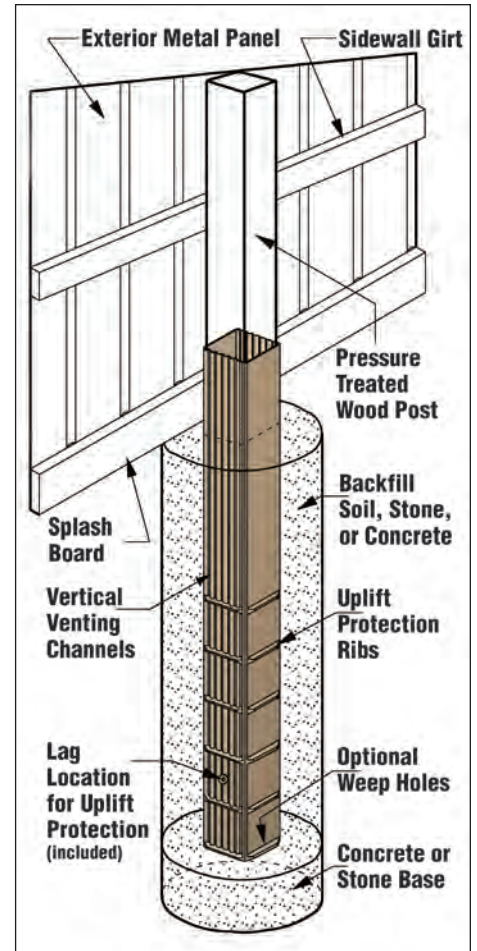
Figure 20. Blow-molded plastic barrier system
