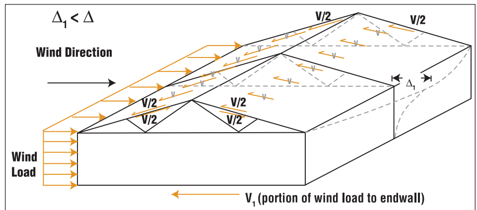
Figure 2. Post-frame building responses to rated loads with diaphragm action. ( \Delta_1 is eave deflection with diaphragm action; \Delta is eave deflection without diaphragm action)
